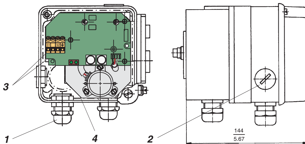
Built-in Position Transmitter Code F
