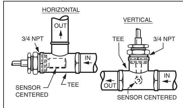
Figure 4. Tee Installations
