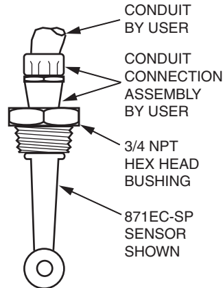
TYPICAL USE WITH BUSHING AND CONDUIT CONNECTION
