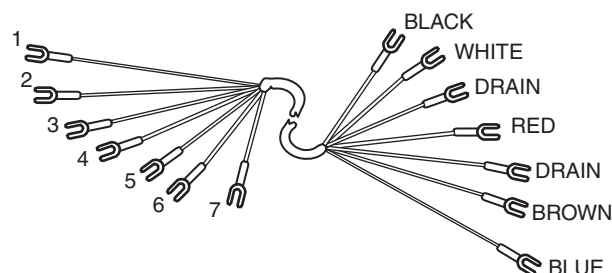
Figure 8. Extension Cable (Foxboro Part 6000130)
