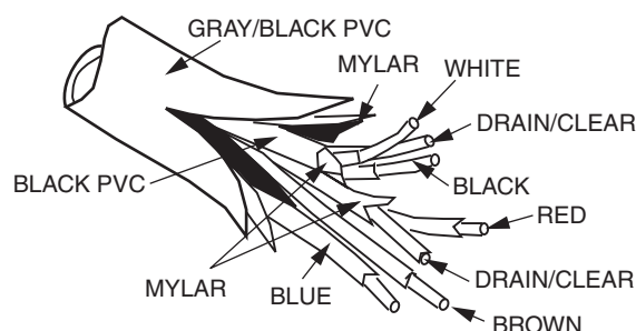
Figure 8. Extension Cable (Foxboro Part 6000130)
