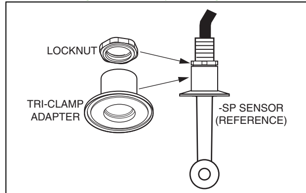
Figure 5. Tri-Clamp Mounting Kit
