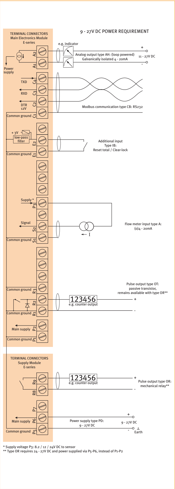
Typical wiring diagram E112-A-AH-CB-IB-OR-PD
