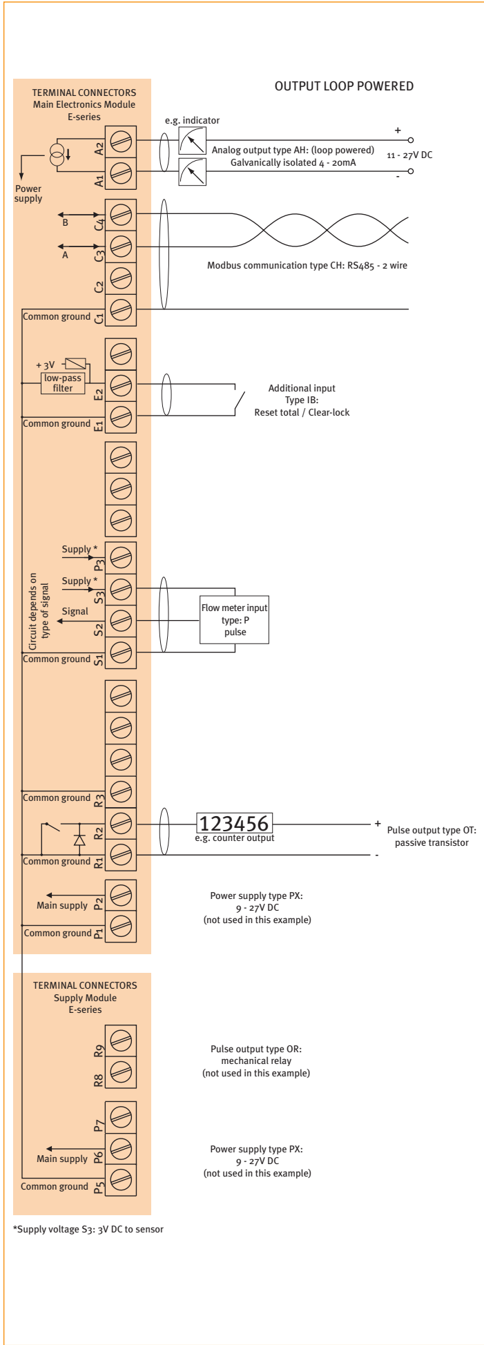
Typical wiring diagram E110-P-AH-CH-IB-OT-PX
