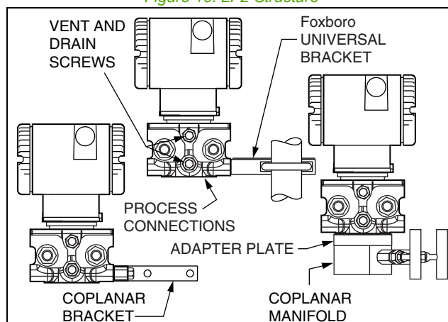
Figure 10. LP2 Structure
