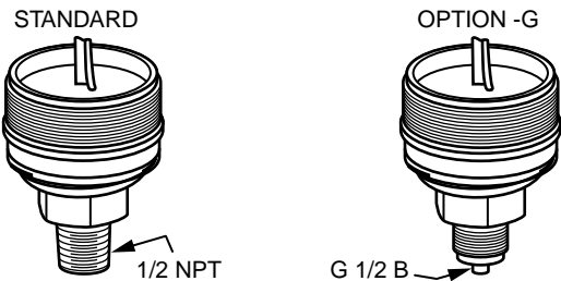
Figure 14. Option -G IAP10/IAP10S/IGP10/IGP10S SPAN LIMIT CODES C, D, E, and F
