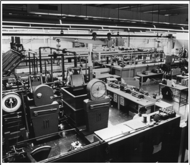
Figure 35. Laboratory Flow Calibration
