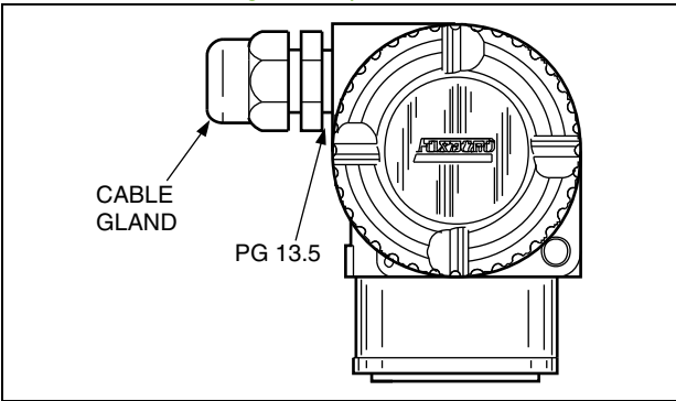
Figure 9. Option -A2
