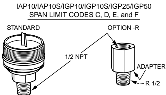
Figure 16. Option -R
