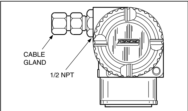
Figure 8. Option -A1
