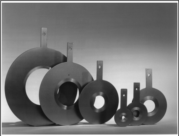
Figure 39. Orifice Plates
