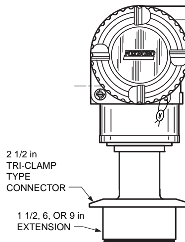
TRANSMITTER WITH INTEGRAL MINI TANK SPUD SEAL TRI-CLAMP TYPE CONNECTOR
