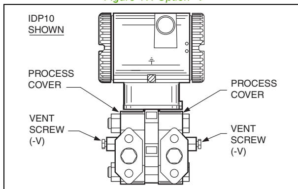
Figure 17. Option -V
