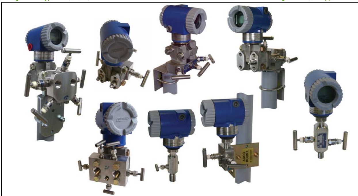
Figure 41. Typical 1-, 2-, 3-, and 5-Valve Manifold/Transmitter Assemblies with AGCO Mounting Bracket, as applicable
