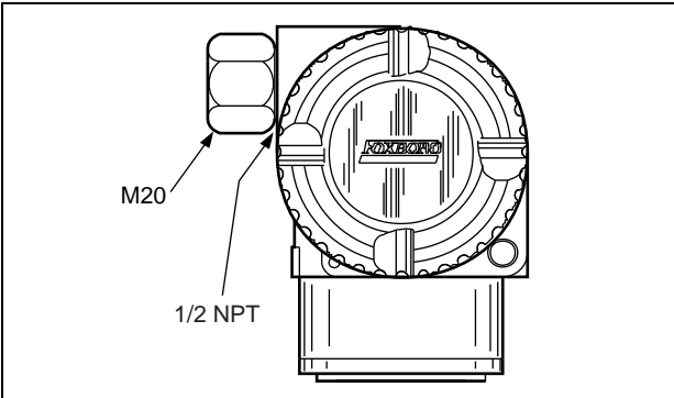
Figure 10. Option -A3
